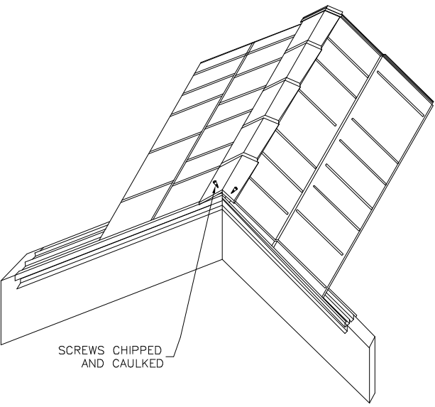
RIDGE CAP
